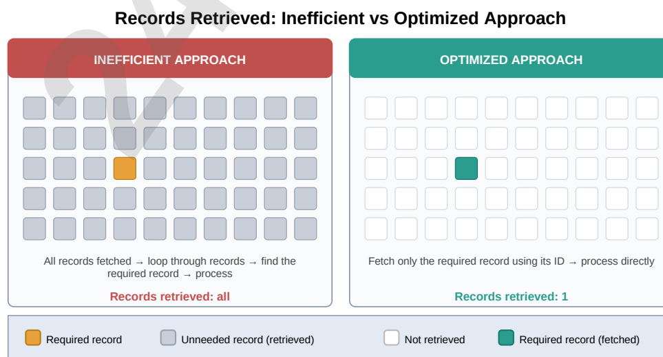
Figure 2: Records Retrieved by the Inefficient and Optimized Approaches (Conceptual Diagram)
